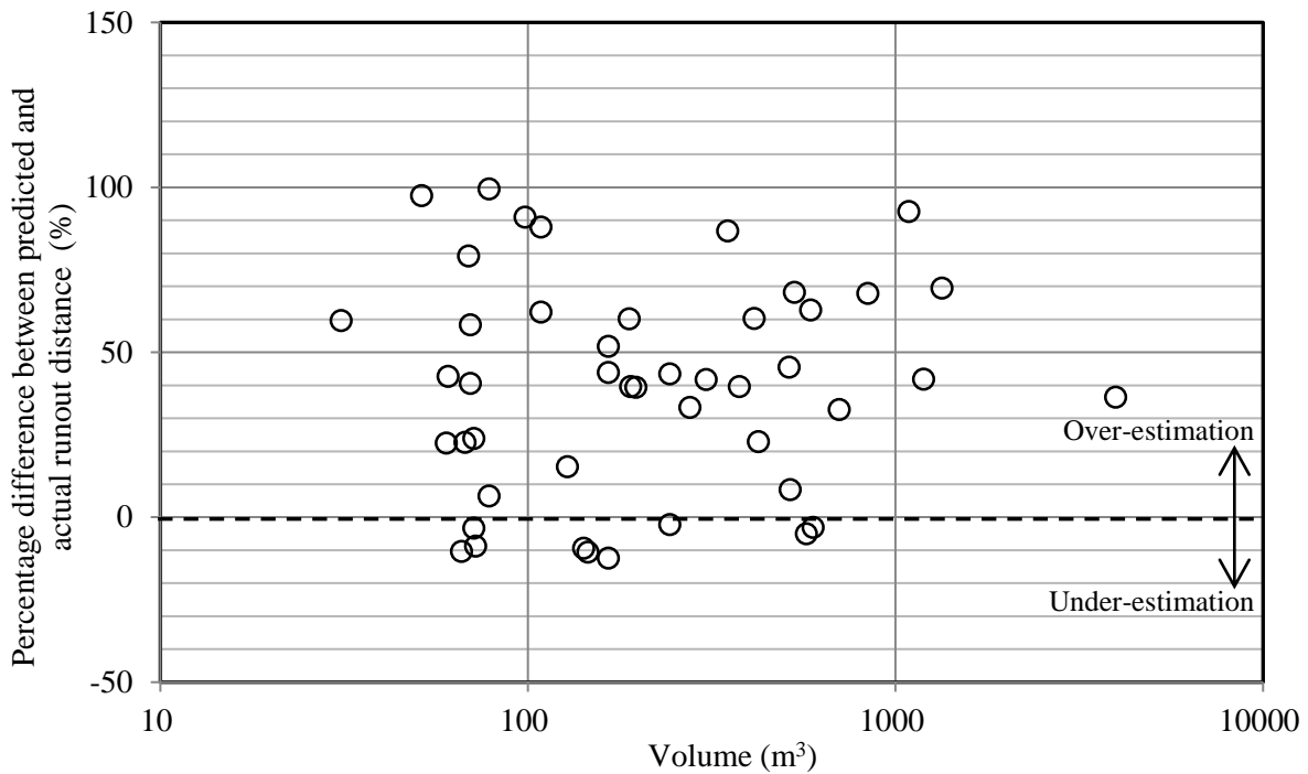
Figure 5 - Prediction of runout distances using \phi_a = 18^\circ , \xi = 1000 \text{ m/s}^2 according to landslide volumes
